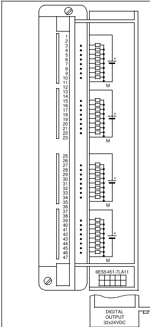
Terminal Assignment
