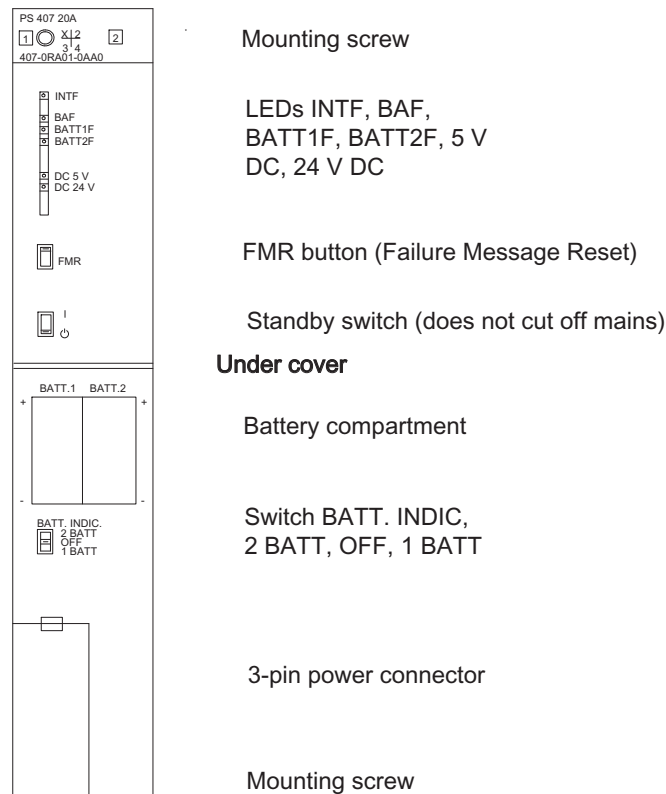
Figure 3-1 Operator controls and indicators on the PS 407 20A power supply module
